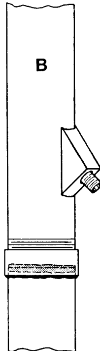
Figure 30. Pitless unit connections for wells with steel well casing pipe. NOTE: A well casing pipe nipple, 1/2 threaded-1/2 beveled may be used in lieu of a full pipe coupling.
