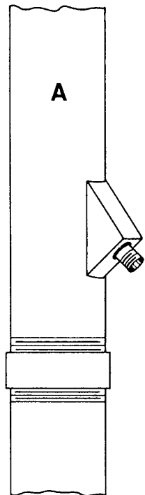
Figure 30. Pitless unit connections for wells with steel well casing pipe. NOTE: A well casing pipe nipple, 1/2 threaded-1/2 beveled may be used in lieu of a full pipe coupling.
