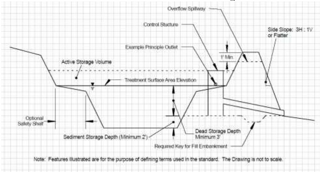
Figure 1 Clarification of Sediment Basin Terminology
