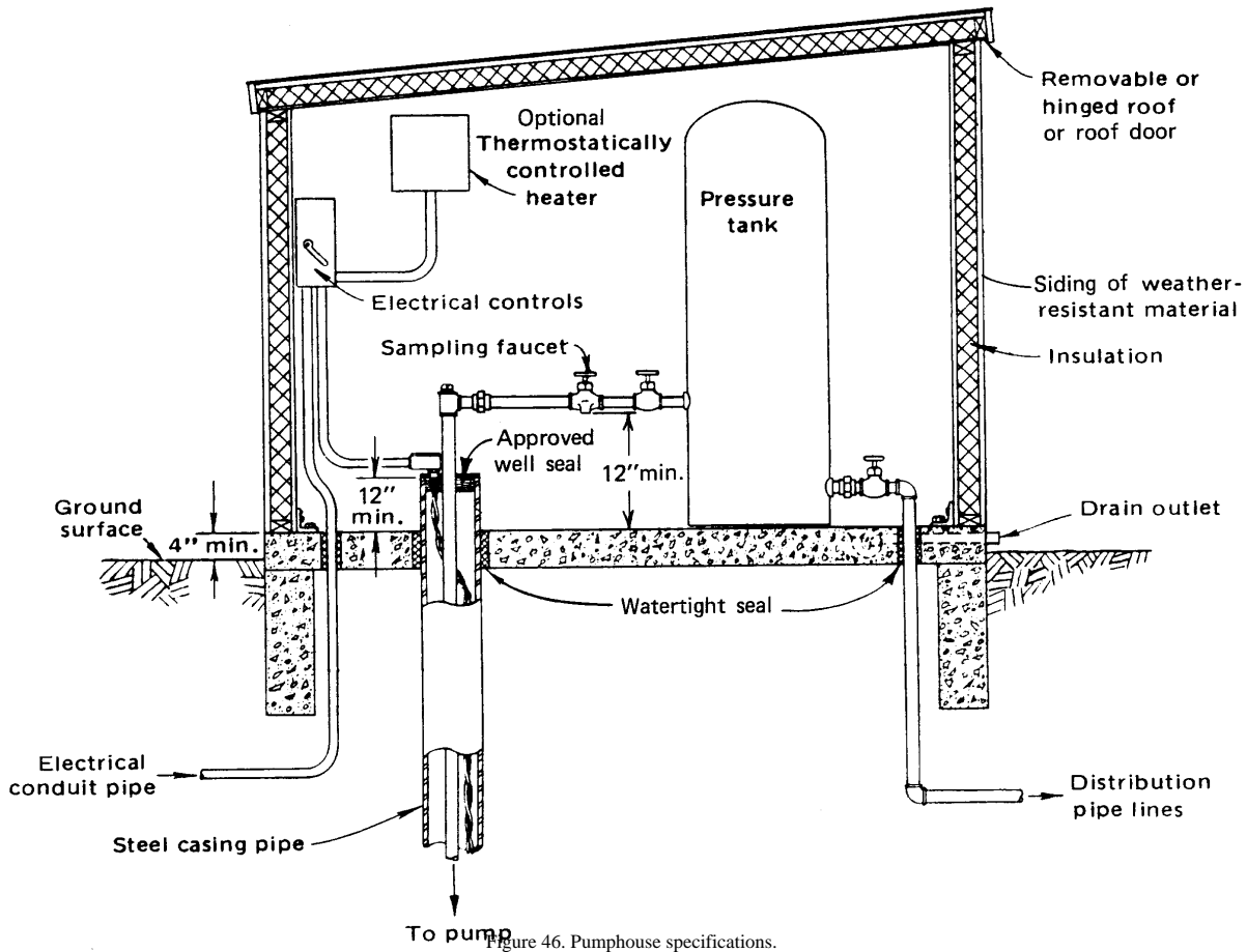
Figure 46. Pumphouse specifications.
